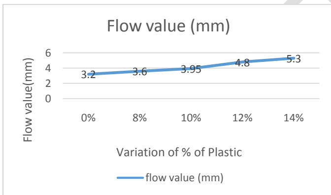
Fig.12 Flow value for different samples of the mix
