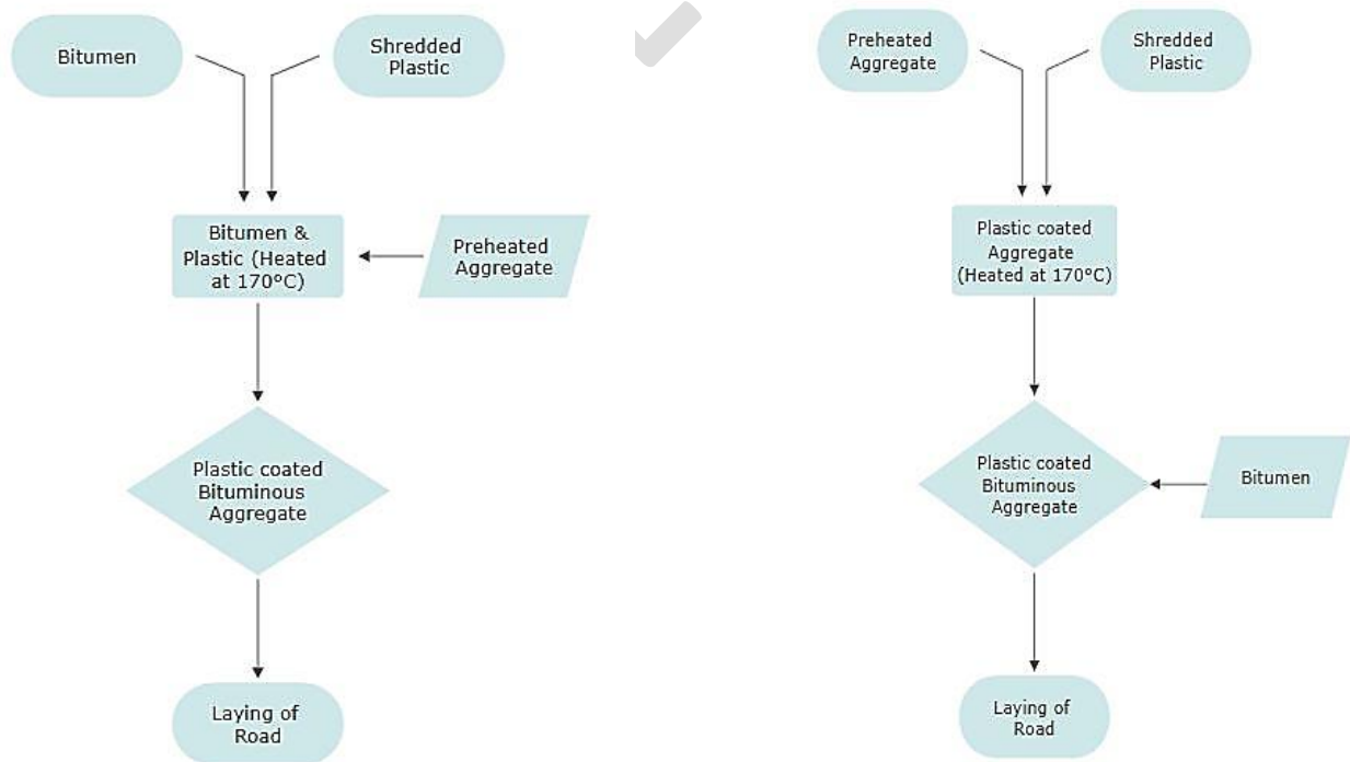
Fig1. Wet Process Fig2. Dry Process
