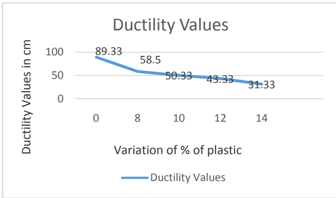
Fig.10 Ductility value for different samples of the mix
