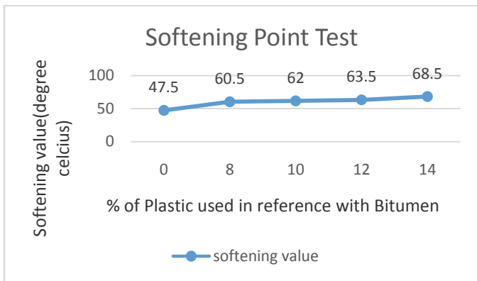
Figure.7 Softening value for different samples of the mix
