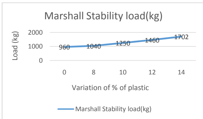
Fig.9 Marshall stability load for different samples of the mix
