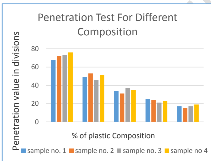
Fig.6 Penetration value for different samples of the mix
