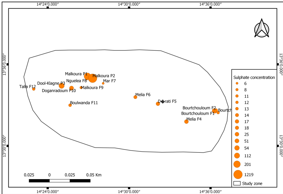
Figure 10. Spatial distribution of sulphate levels in the zone
