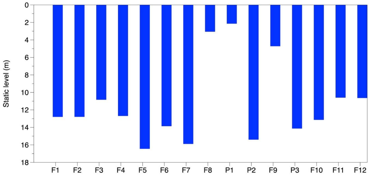
Figure 4. Static levels at sampled water points
