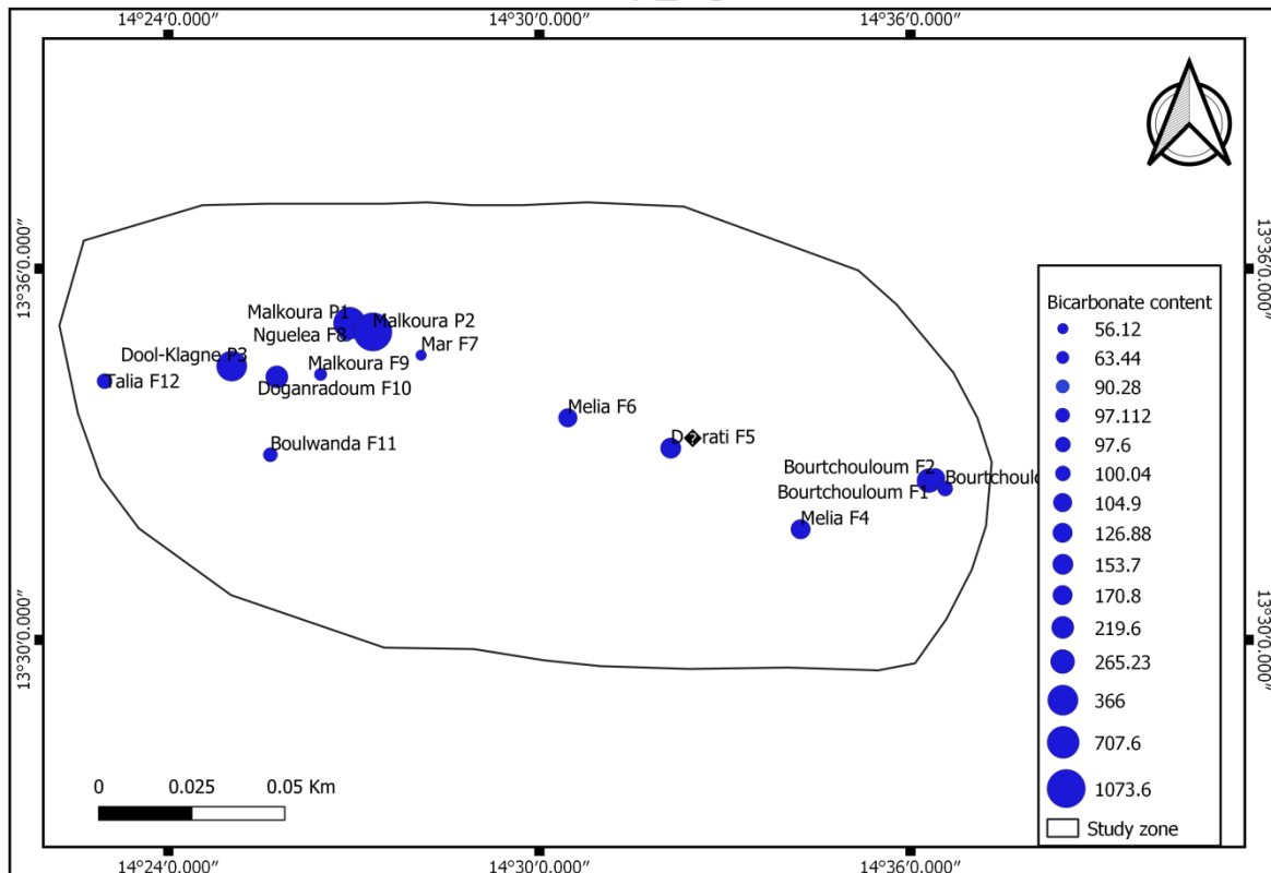
Figure 9. Spatial distribution of bicarbonate levels in the study area
