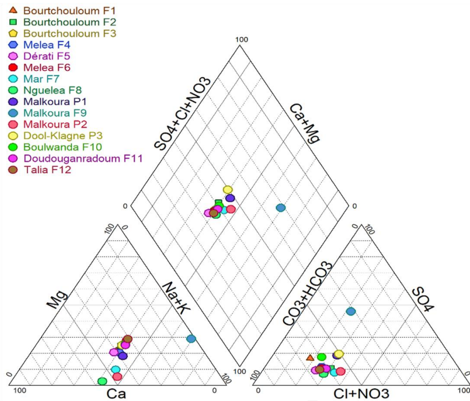
Figure 6. Water chemistry facies
