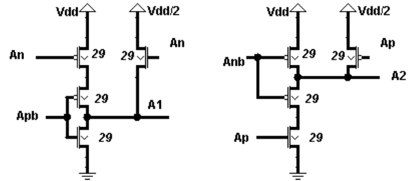
Fig. 5. A^1 and A^2 circuits
