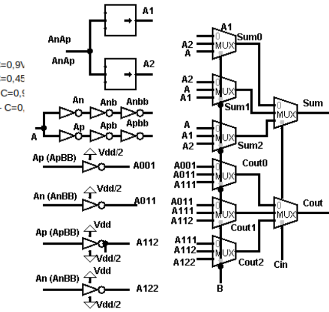
Fig. 14. Balanced ternary adder - Version 1
