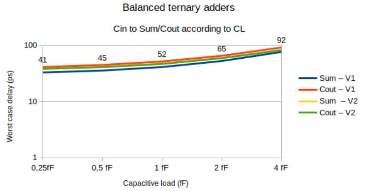
Fig. 18. C_{in} to Sum/ C_{out} of balanced ternary adders according to CL
