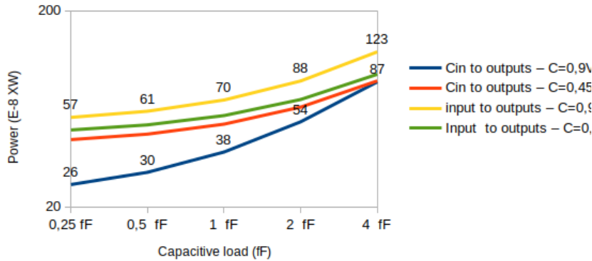
Power dissipation according to CL
