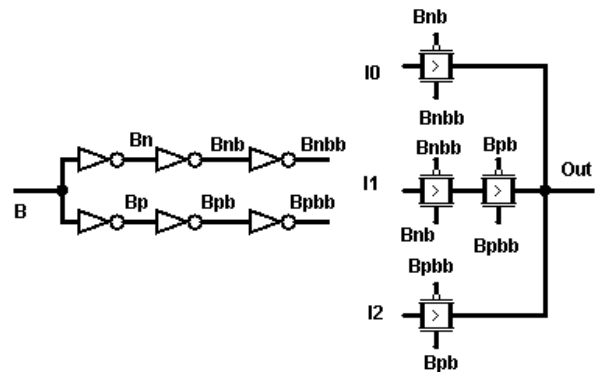
Fig. 6. 3-input MUX with ternary control
