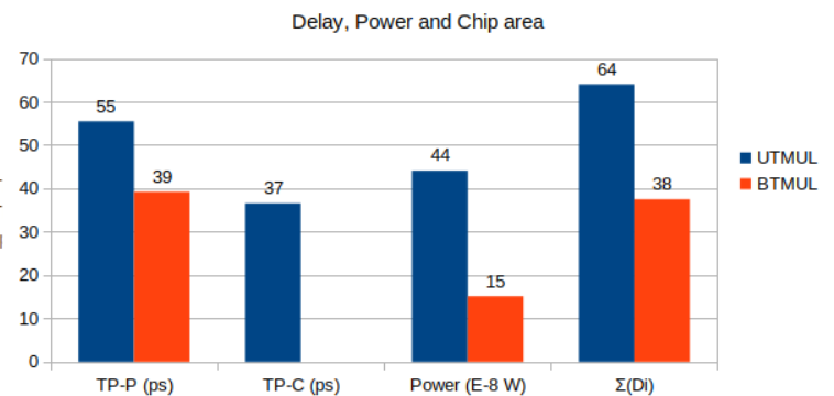
Fig. 24. Unbalanced and Balanced 1-trit multiplier with 2fF capacitive loads
