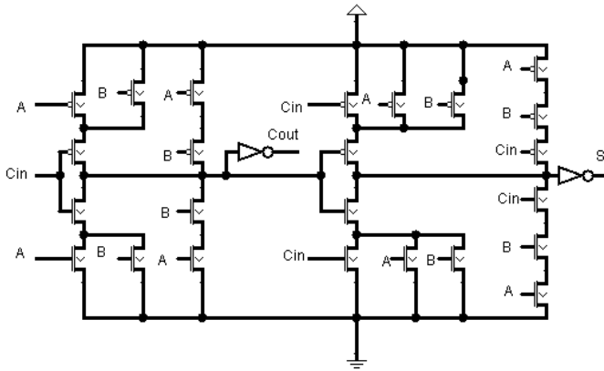
Fig. 7. 28T binary full adder
