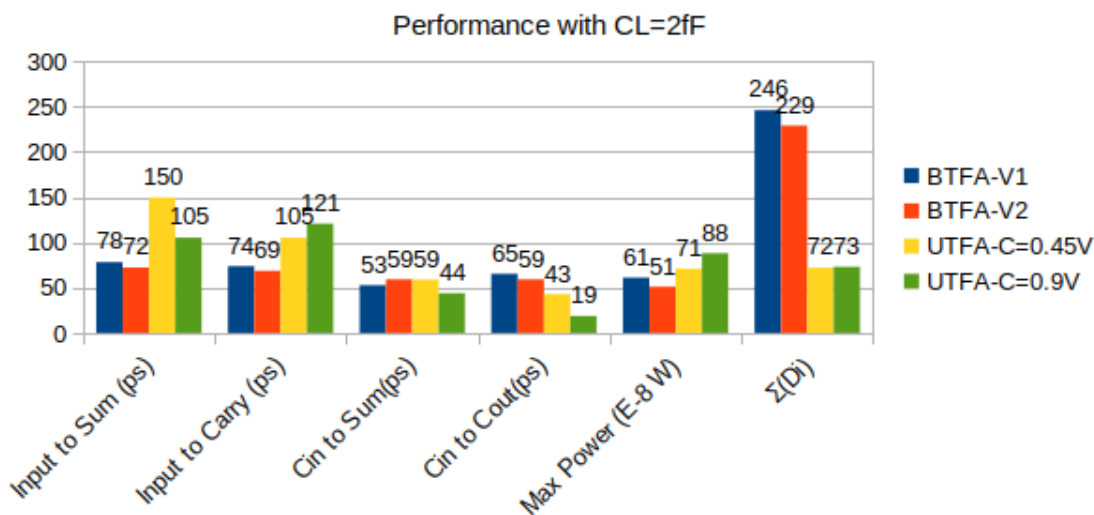
Fig. 20. Comparing 1-trit balanced and unbalanced adder (CL=2fF)
