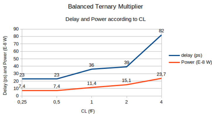
Fig. 23. Balanced ternary multiplier performance according to CL
