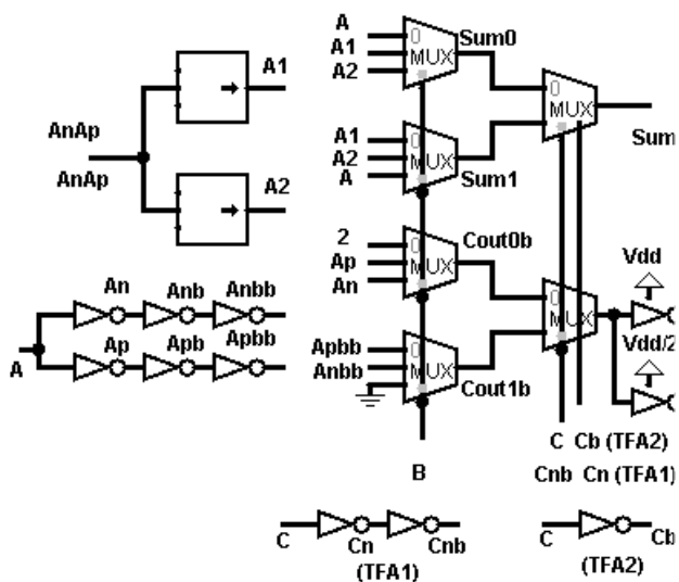
Fig. 9. Unbalanced 1-trit Full Adder (Mux approach)
