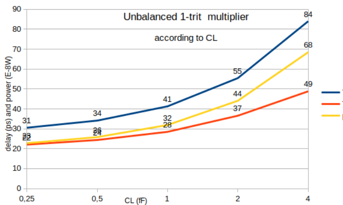
Fig. 22. Unbalanced ternary multiplier performance according to CL
