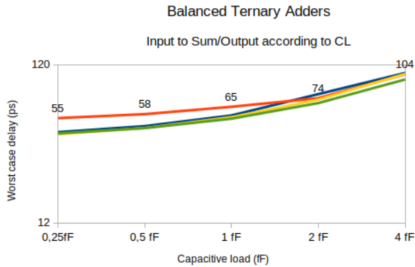
Fig. 17. Input to Sum/ C_{out} of balanced ternary adders according to CL
