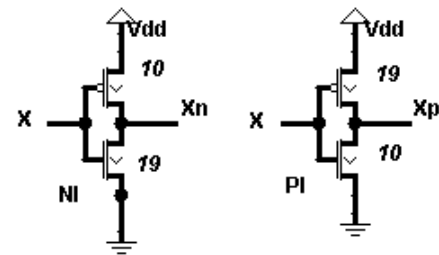
Fig. 4. Threshold detectors
