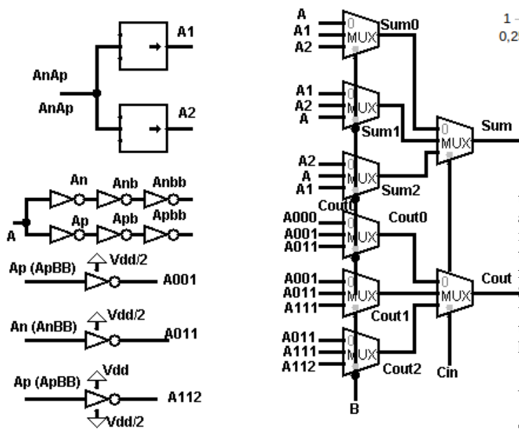
Fig. 10. Unbalanced Ternary (3,2) counter
