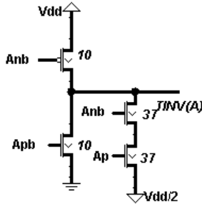
Fig. 16. Ternary inverter
