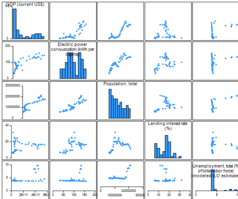
Fig 3. SCATTERPLOT MATRIX
