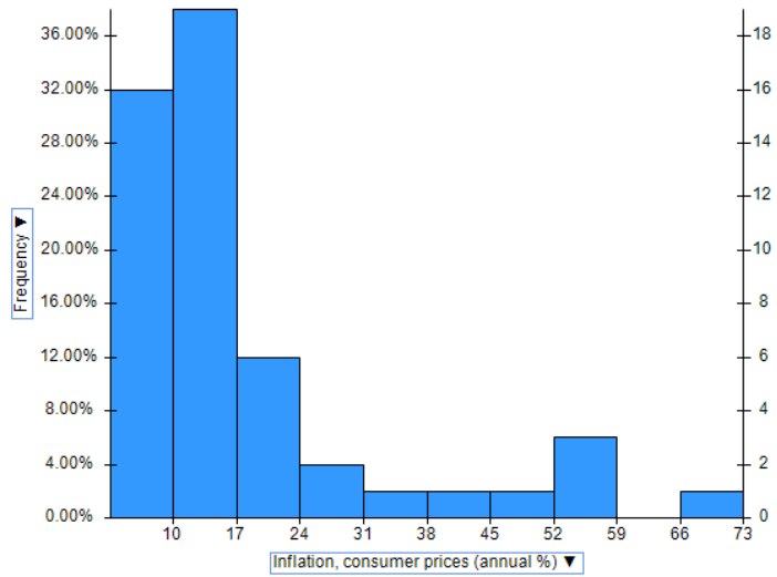
Fig 2.HISTOGRAM
