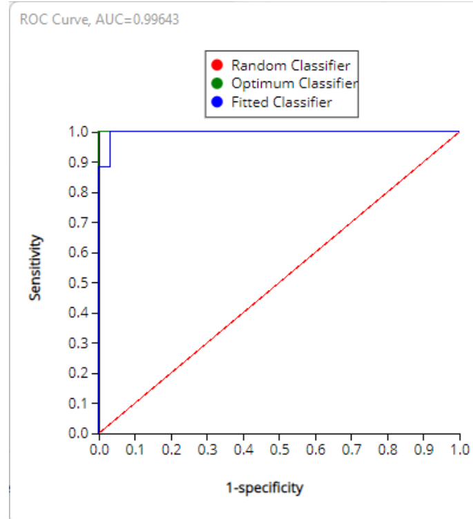
Chart 2.ROC CURVE
