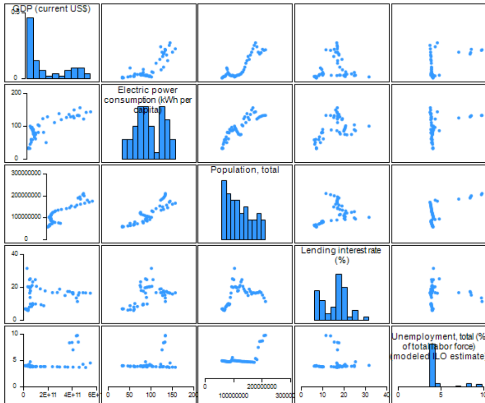
Fig 3. SCATTERPLOT MATRIX
