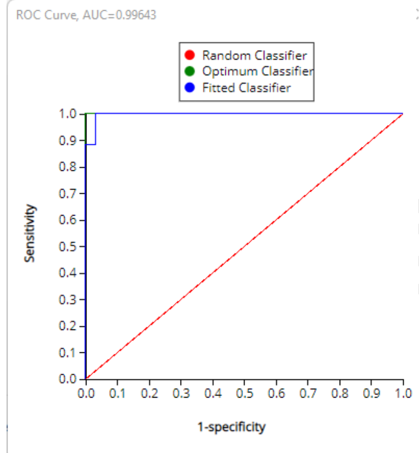
Chart 2.ROC CURVE
