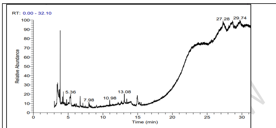
Figure 9 The GC-MS chromatogram of the ethanolic fraction of T. terrestris fruit
