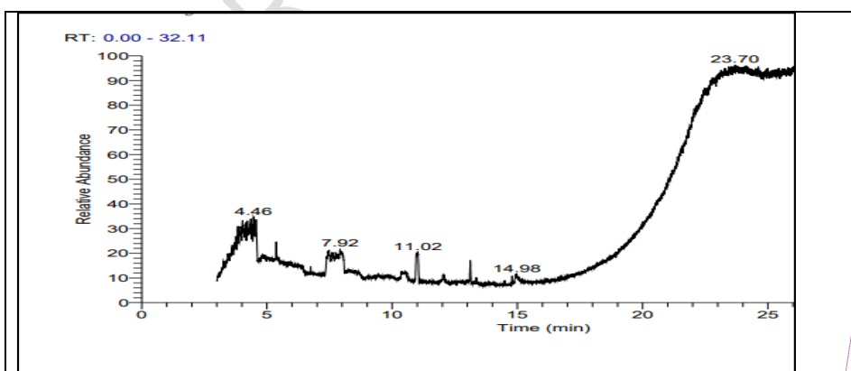
Figure8 The GC-MS chromatogram of the ethanolic fraction of T. terrestris leaves
