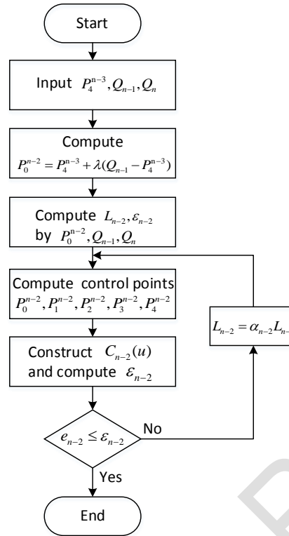
Fig.10.Flowchart of Routine 3
