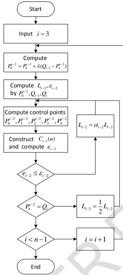
Fig.9.Flowchart of Routine 2
