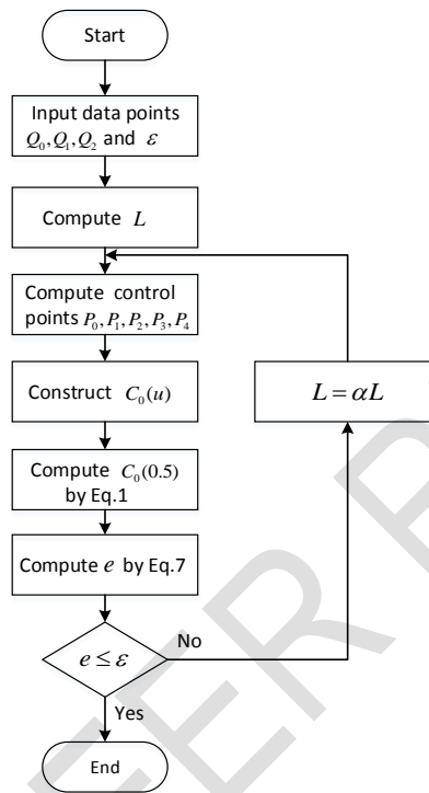
Fig.4. Computing routine to adjust the approximation error
