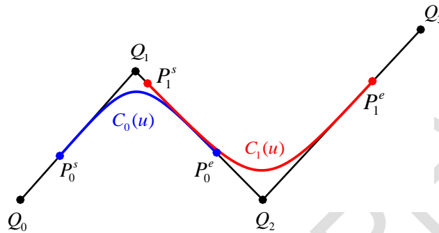
Fig.6.The overlapping phenomenon between transition curves
