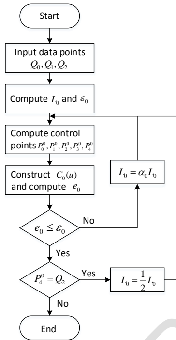
Fig.8.Flowchart of Routine 1
