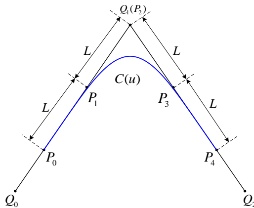
Fig. 1. Transition curve
