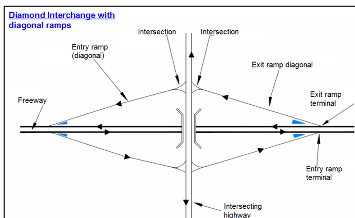
Figure 5a: Example of 4-leg service interchange components (diamond with diagonal ramps).
