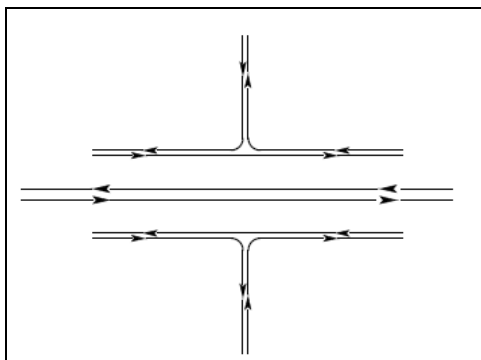
Figure 8: Connection to service road.
