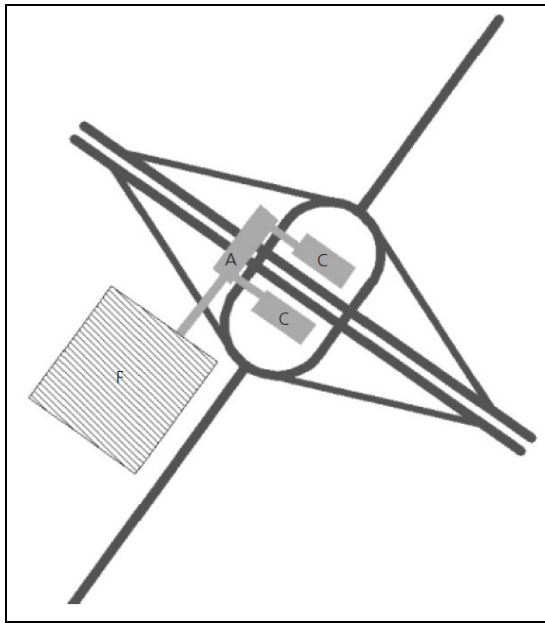
A: Interchange point and passenger facilities on new motorway overbridge; C: Online bus stopping areas and passenger facilities; F: Park and ride facilities.
