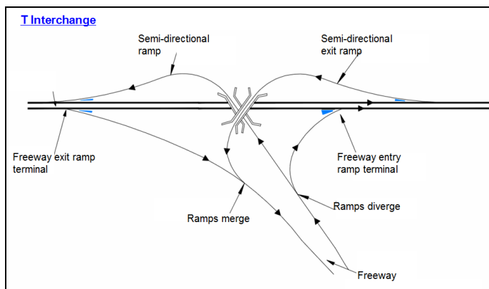
Figure 4 : Examples of 3-leg interchange components ( T interchange).
