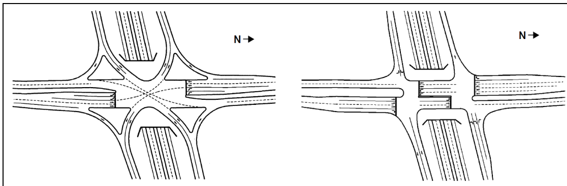
Figure 2: Single point diamond (left) Vs. tight urban diamond interchange (right), [Selinger and Sharp 2000].
