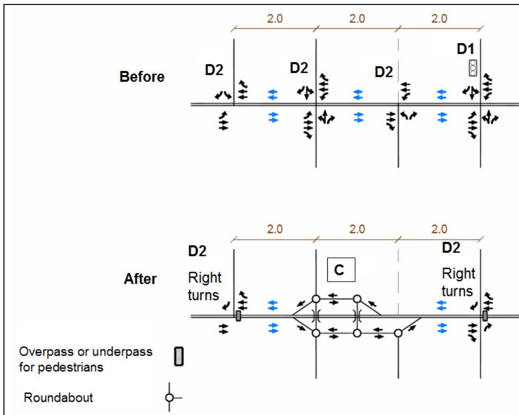
Figure 9: Typical example of system improvements of traffic flow along a major (two-way divided) highway with compact grade separated junction.
