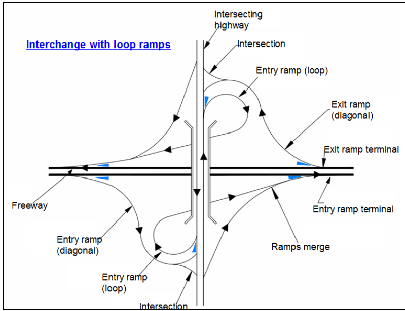
Figure 5b: Example of 4-leg service interchange components with loop ramps.
