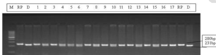
Fig.(4): PCR amplification of seedlings of F 1 generation using gene-specific marker Sub1BC2. M -100 bp DNA ladder. RP - Recurrent parent; D - Donor. Lanes:1-10 = F 1 plants from ADT 36 x CR Dhan 801 cross. Lanes-11-17 = F 1 plants from ADT37 x CR dhan 801 cross.
