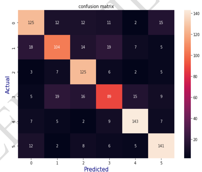
Figure 16: Confusion Matrix of LSTM
