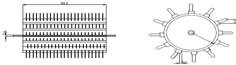
Fig 1: front and Side View of Threshing Cylinder
