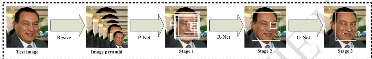
Figure 3: MTCNN network architecture[12].
