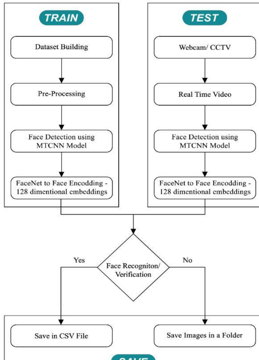
Figure 1: Framework of the Proposed System
