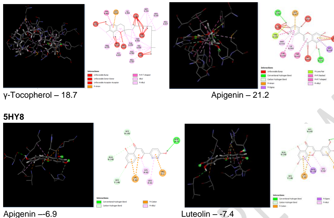
Figure 1: Hydrogen bonding interactions of few compounds with highest score against the proteins
