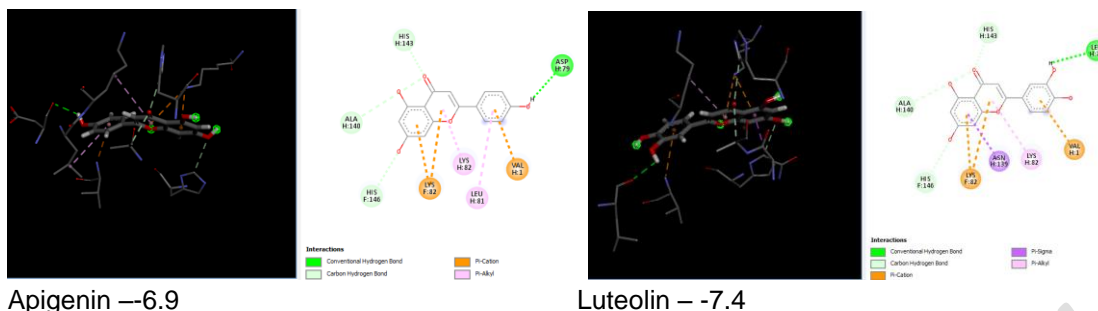
Figure 1: Hydrogen bonding interactions of few compounds with highest score against the proteins
