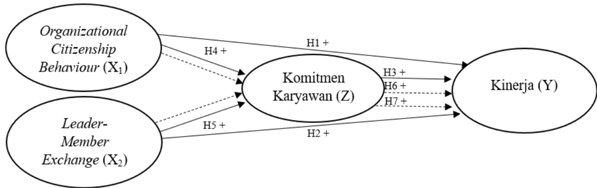
Figure 1 Framework methodology
