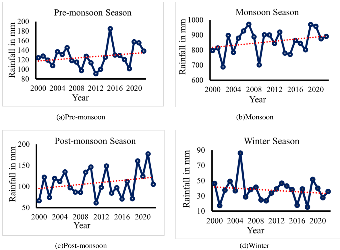
Figure 2: Linear trends for the rainfall in India for the (a.) pre-monsoon, (b.) monsoon, (c.) post-monsoon, and (d.) winter seasons. The solid blue line represents the rainfall data while the red dashed line represents the linear trend.
