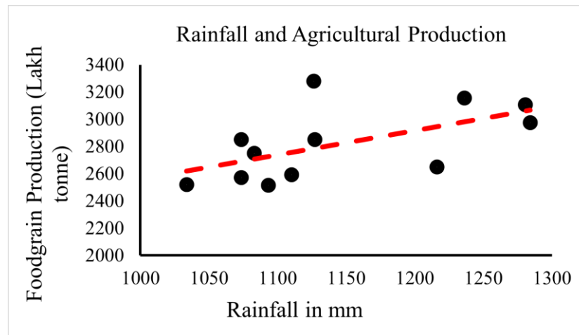
Figure5:Therelationshipbetweenrainfallinmmandthefoodgrainproductiontotal inIndia(lakhtonne).hesymbolsrepresentthedatausedinthepresentworkwhilethe dashed line represents the trend between rainfall and agricultural production.
