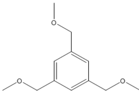
Figure 3: 1, 3, 5-Trimethoxymethylbenzene (TMMB)
