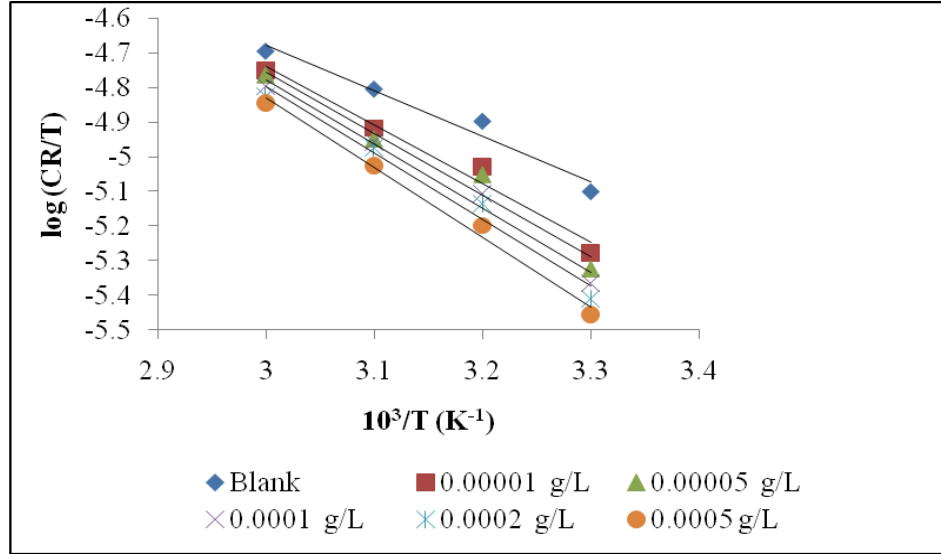
Figure 6: Transition State plot for mild steel coupons in 1M HCl in the absence and presence of different concentrations of TMMB.
