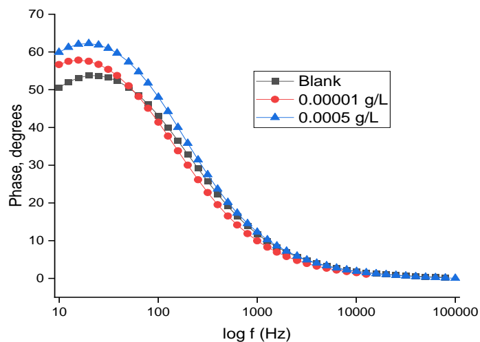
Figure 11: Bode Plot of mild steel in 1.0 M HCl solution in the absence and presence of different concentrations of TMMB at 303 K.
