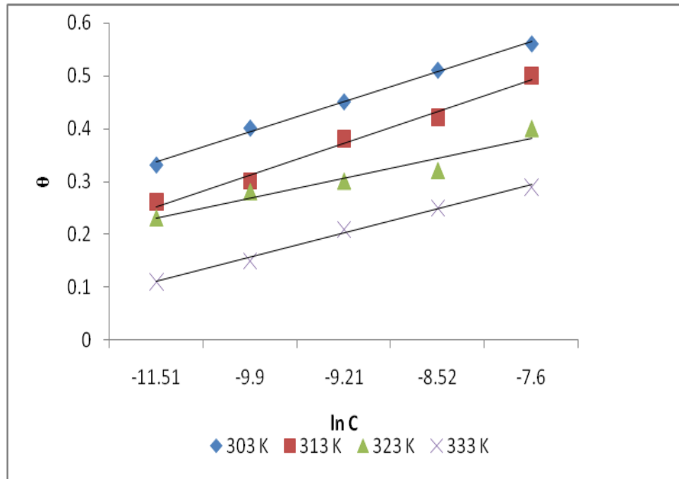
Figure 7: Temkin adsorption isotherm for mild steel corrosion in 1 M HCl solution in the absence and presence of different concentrations of TMMB.
