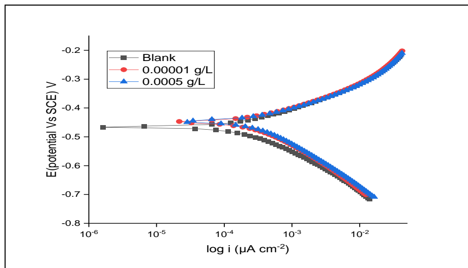
Figure 8: Polarization curve of mild steel in 1.0 HCl solution in the absence and presence of different concentrations of TMMB at 303 K.
