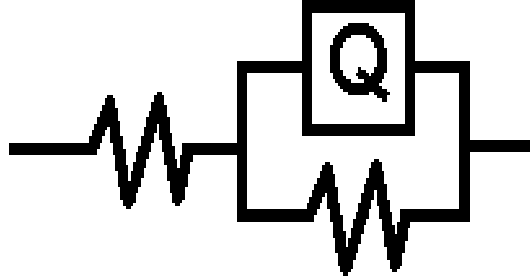
Figure 9: One time constant phase element (CPE) circuit
