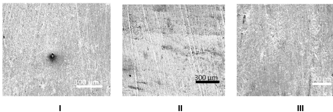
Figure 12: SEM image of mild steel surface exposed to (I) 1.0 M HCl solution (blank), (II) 1.0 M HCl containing 0.1 \times 10^{-4} \text{ gL}^{-1} of TMMB, and (III) 1.0 M HCl containing 5.0 \times 10^{-4} \text{ gL}^{-1} of TMMB.
