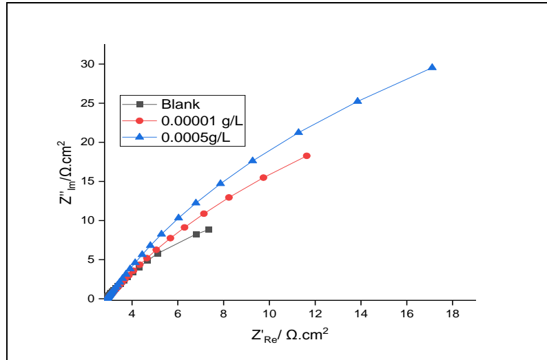
Figure 10: Nyquist plot of mild steel in 1.0 HCl solution in the absence and presence of different concentrations of TMMB at 303 K.
