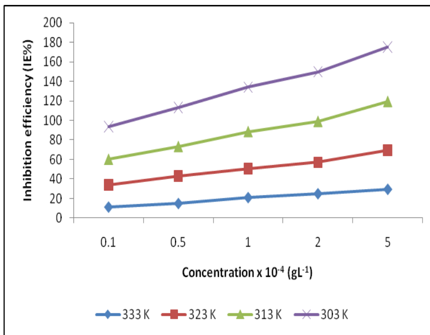
Figure 4: Effect of 1, 3, 5-trimethoxymethylbenzene (TMMB) on the corrosion inhibition efficiency of mild steel at different temperatures.
