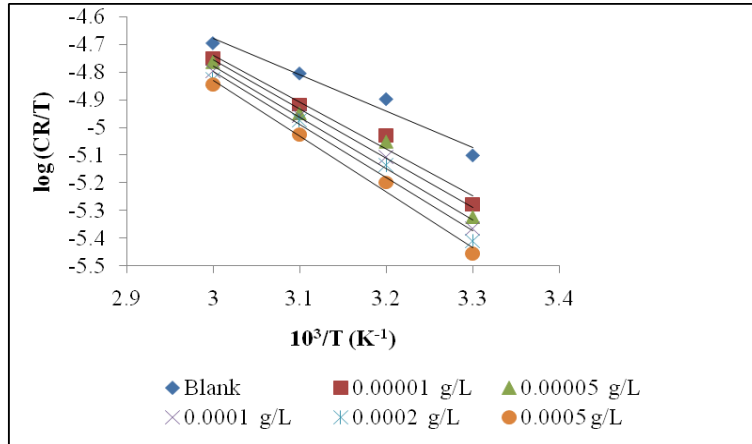
Figure 4: Transition State plot for mild steel coupons in 1M HCl in the absence and presence of different concentrations of TMMB.
