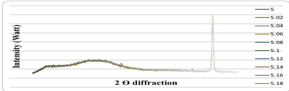
Fig. 15 X-Ray Diffraction of the Potato Starch Film
