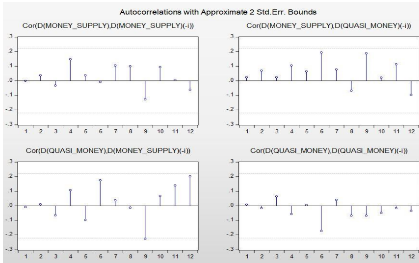
Figure 3: Correlogram of Residuals of the BVAR(2) Model
