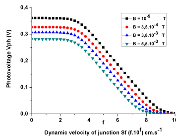
Figure 4: Photovoltage versus dynamic junction velocity for different magnetic field values ( \lambda = 940\mu\text{m} ; D_n = 26\text{cm}^2 ; Sb = 10^2\text{cm.s}^{-1} ; L_n = R = 50\mu\text{m} ; H = 100\mu\text{m} ).
