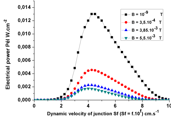
Figure 5: electrical power as a function of the dynamic velocity at the junction for different values of the magnetic field ( D_n = 26\text{cm}^2 ; Sb = 10^2\text{cm.s}^{-1} ; L_n = R = 50\mu\text{m} ; H = 100\mu\text{m} ).
