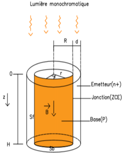
Figure 1: Physical model of the radiale Radial junction cell model
