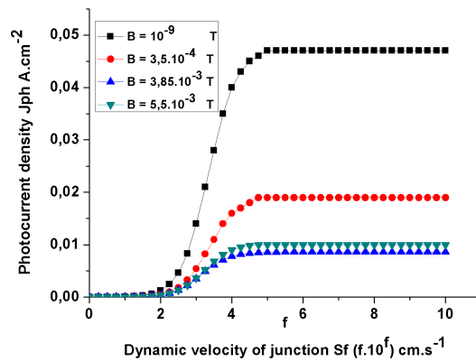
Figure 3: Photocurrent density as a function of dynamic velocity at the junction for different magnetic field values ( \lambda = 940\mu\text{m} ; D_n = 26\text{cm}^2 ; Sb = 10^2\text{cm.s}^{-1} ; L_n = R = 50\mu\text{m} ; H = 100\mu\text{m} ).
