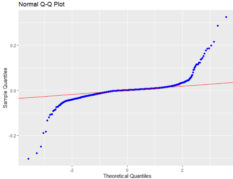
Figure 6: Normal Q-Q Plot
