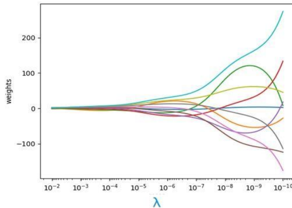
Fig. 2. Ridge Coefficient Path
