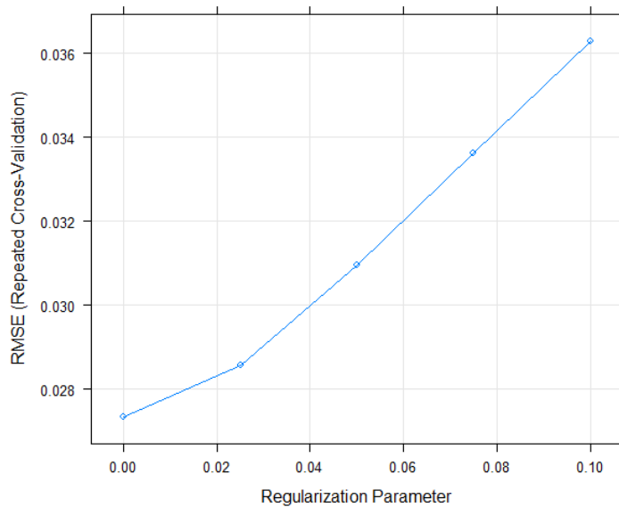
Fig. 7. Ridge tuning parameter plot of regularization
