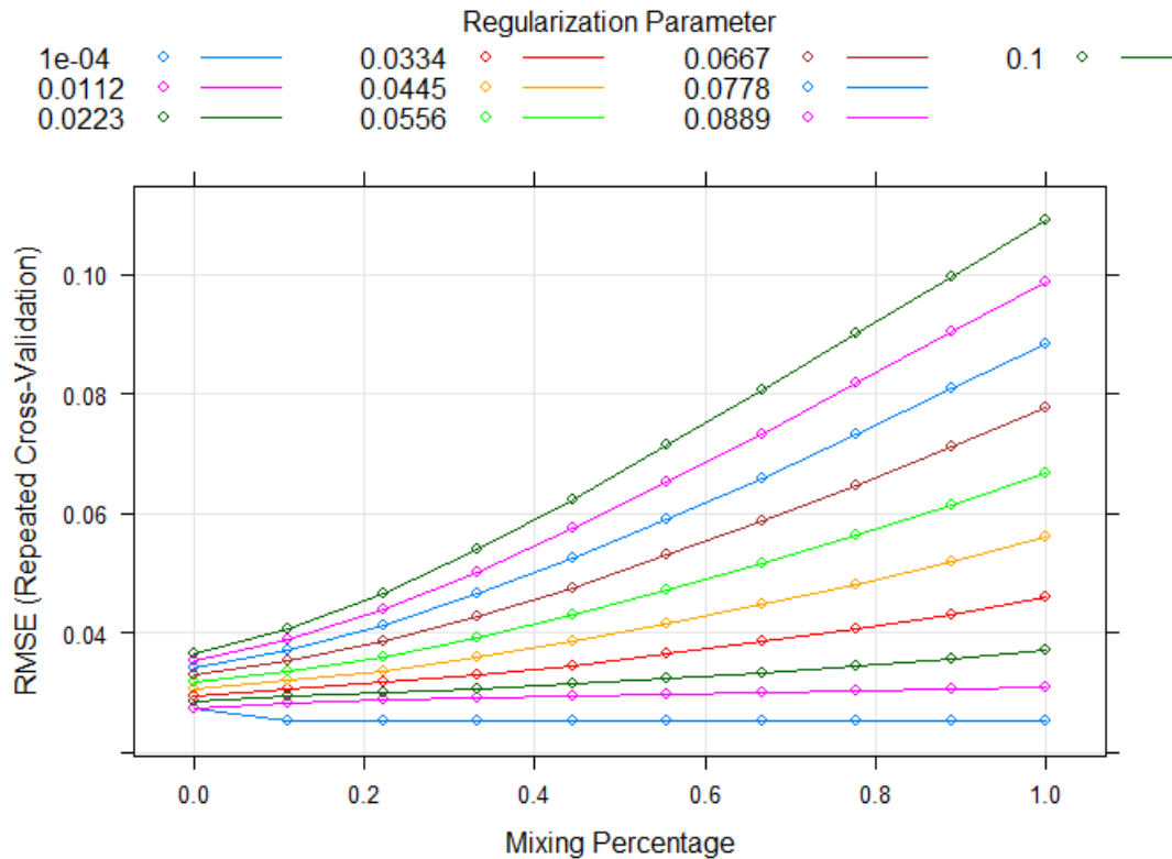
Fig. 11. The 10-fold cross validation RMSE across 10 alpha values (x-axis) and 10 lambda values (line colours)
