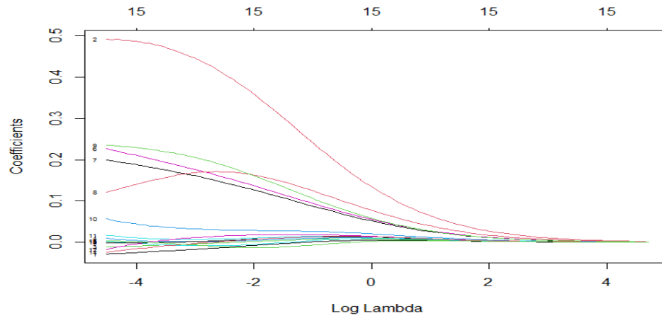
Fig. 8. Normalized Model Coefficients vs. Lambda Hyperparameter
