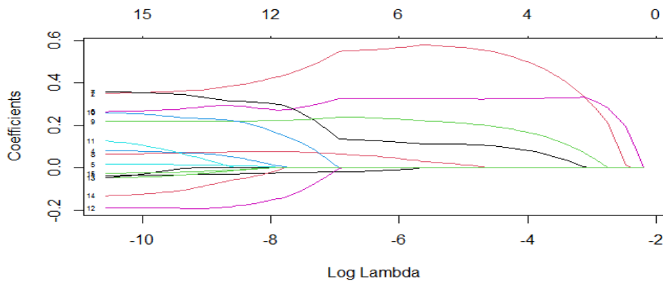
Fig. 9. Standardized Model Coefficients vs. Lambda Hyperparameter
