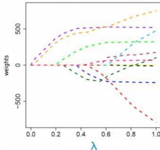
Fig. 3. LASSO Coefficient Path
