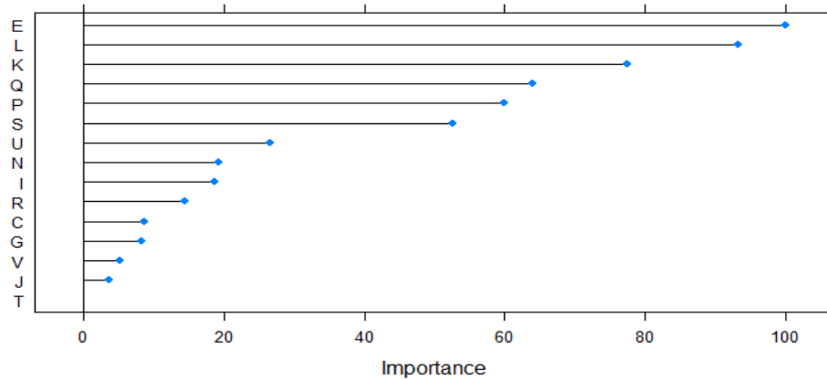
Fig. 10. Variable Importance Plot
