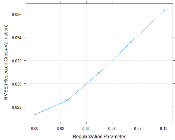
Figure 7 Ridge tuning parameter plot of regularization.
