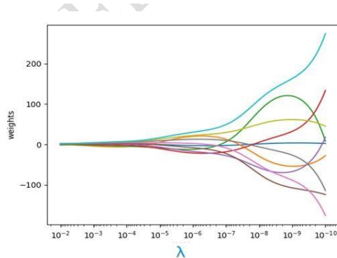
Figure 2: Ridge Coefficient Path
