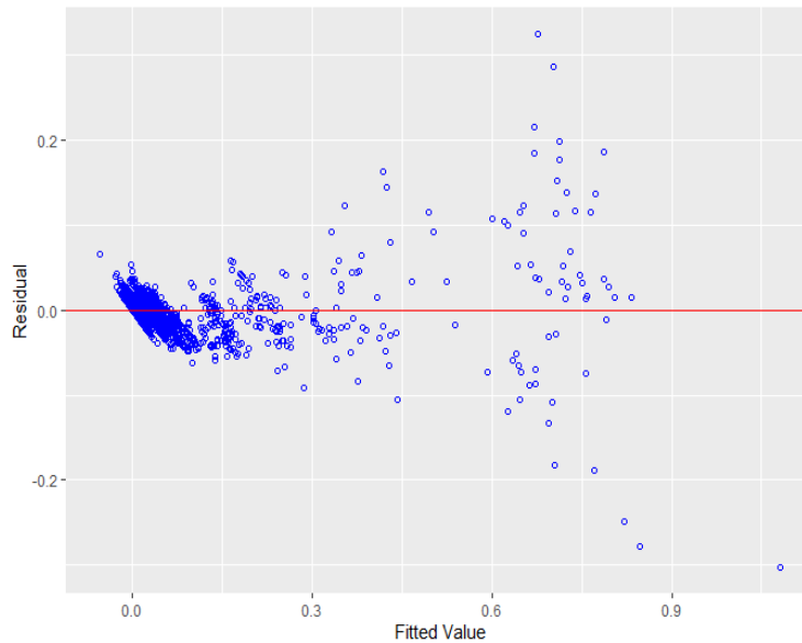
Figure 5: Scatterplot of residuals vs fitted values
