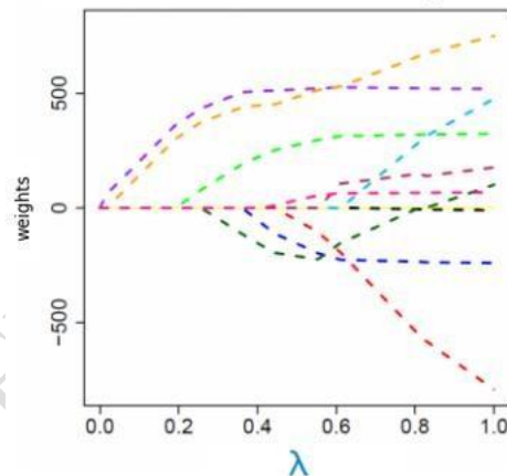
Figure 3: LASSO Coefficient Path
