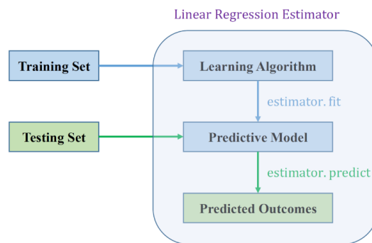
Figure 1: Regression, machine learning block diagram
