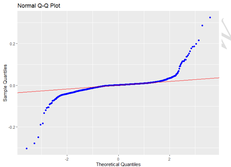
Figure 6: Normal Q-Q Plot
