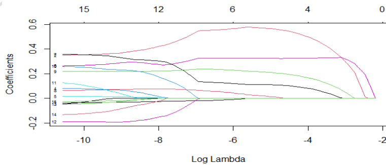
Figure 9: Standardized Model Coefficients vs. Lambda Hyperparameter
