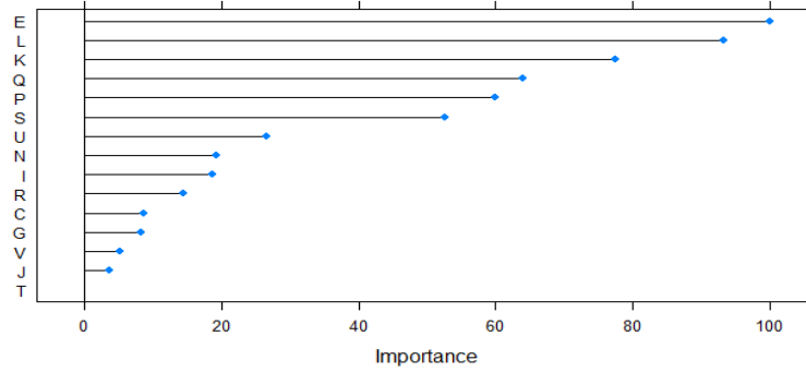
Figure 10 Variable Importance Plot
