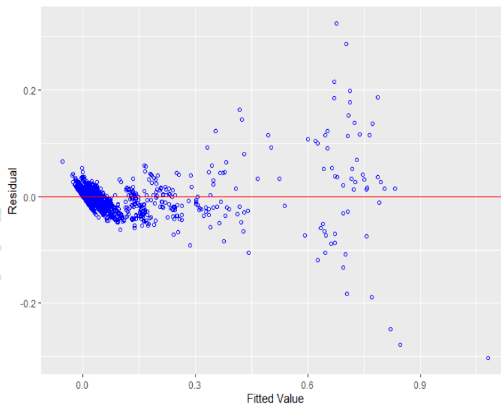
Fig. 5. Scatterplot of residuals vs fitted values
