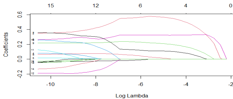
Fig. 9. Standardized Model Coefficients vs. Lambda Hyperparameter
