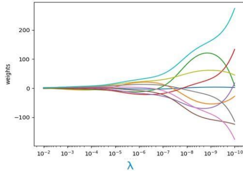
Figure Fig. 2. Ridge Coefficient Path
