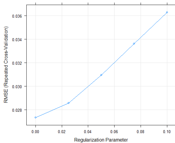
Figure 7. Ridge tuning parameter plot of regularization.
