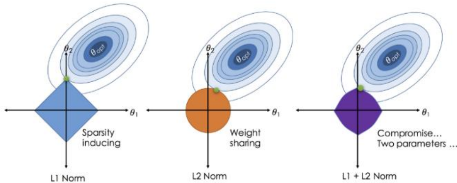
Figure 4: Differences between L1, L2 and L1+L2 norm
