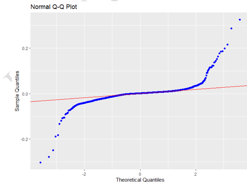
Figure 6: Normal Q-Q Plot
