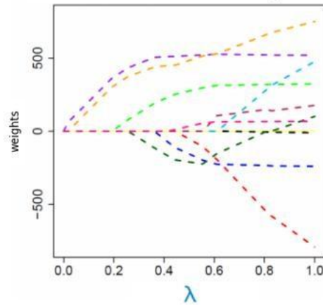
Figure-3: LASSO Coefficient Path
