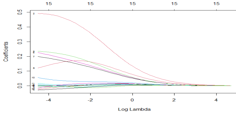
Figure 8 Normalized Model Coefficients vs. Lambda Hyperparameter
