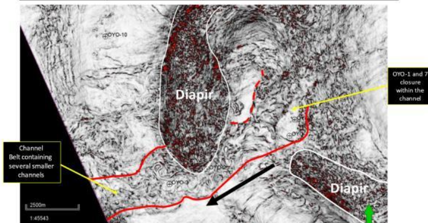
Figure 4. Compartmentalised Channel.
