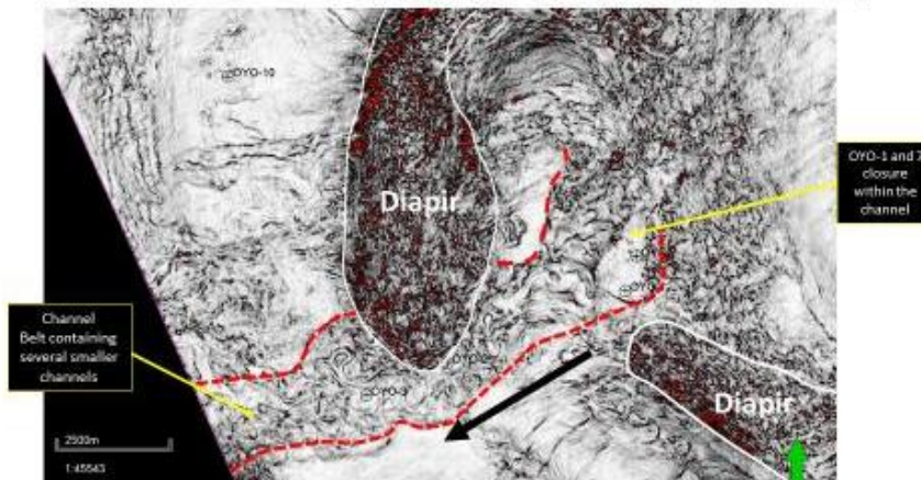
Figure 9. X2 Channels showing producing wells within the channels OYO 10 located on the Floodplain.
