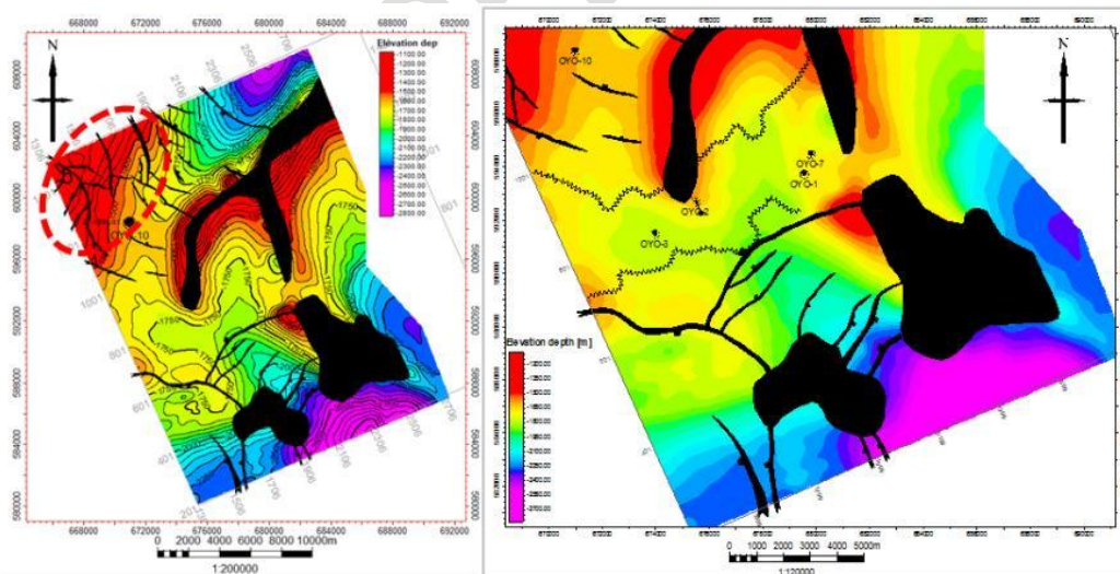
Figure 11.X2 Channel Trap Mechanism.
