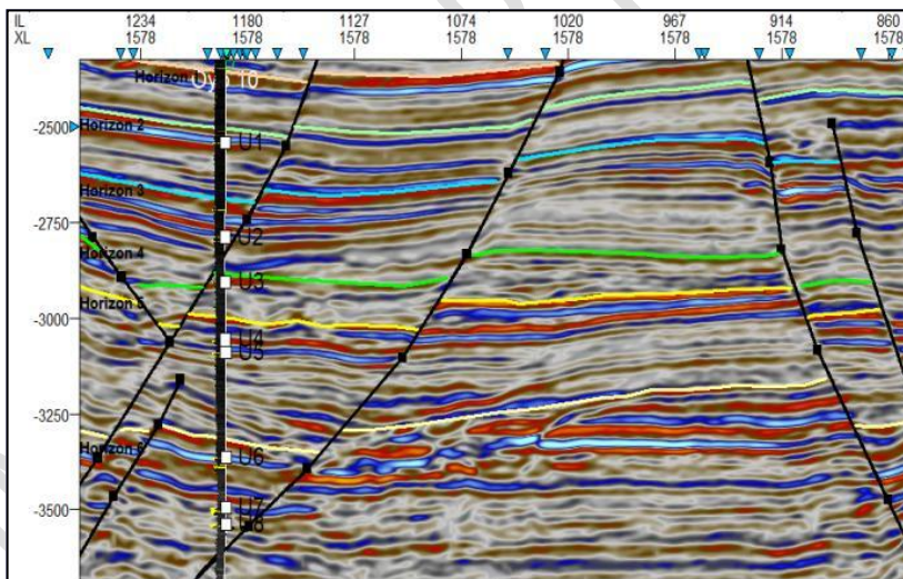
Figure 6. Welltop to seismic mach.
