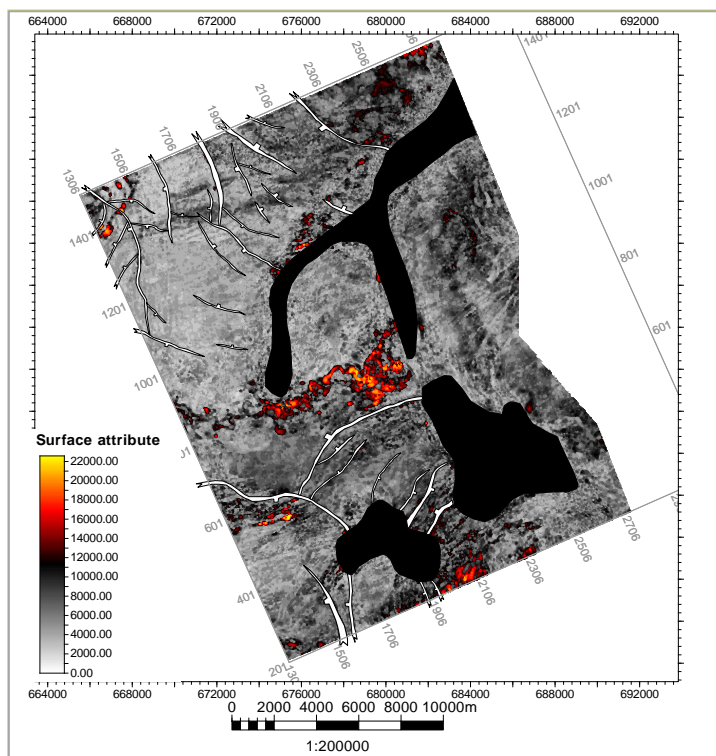
Figure 10. Diapir and faulting zone as a trapping mechanism.
