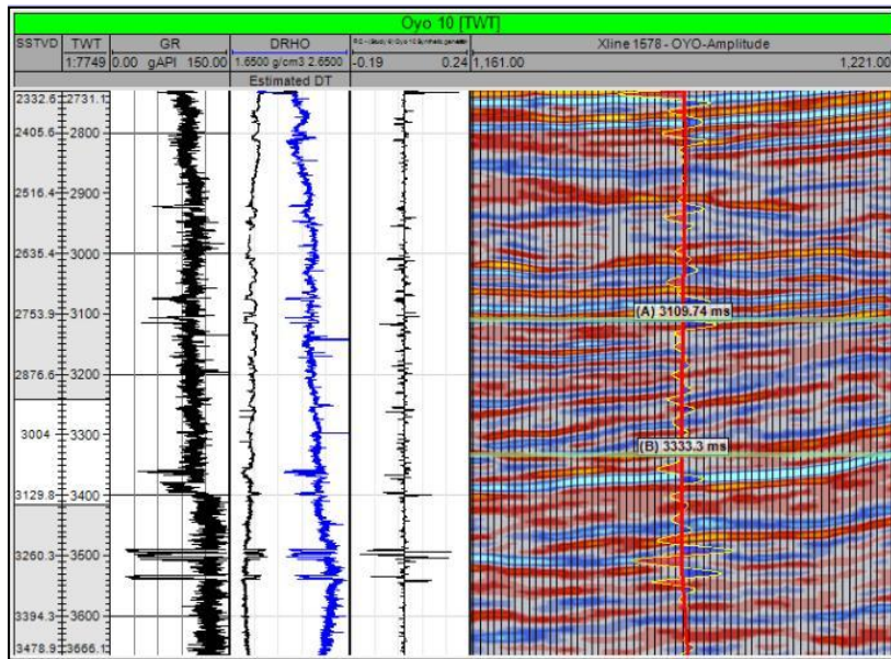
Figure 5. Synthetic Seismogram Generation.
