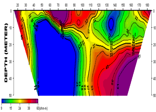
Profile (2-D Resistivity Structure)
