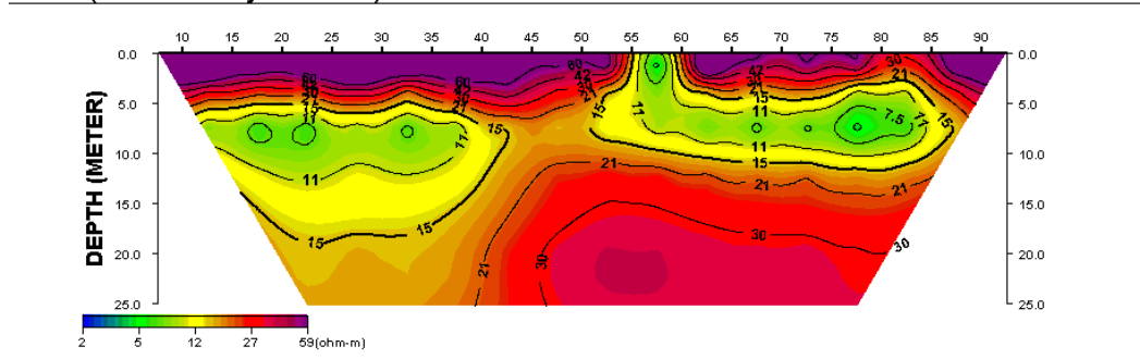
Figure 5. 2D resistivity Images
