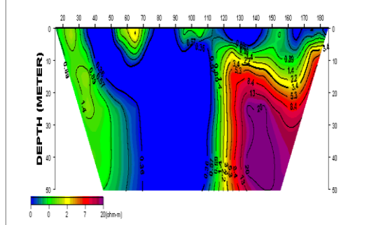
Profile (2-D Resistivity Structure)
