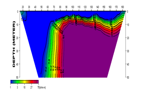
Profile (2-D Resistivity Structure)
