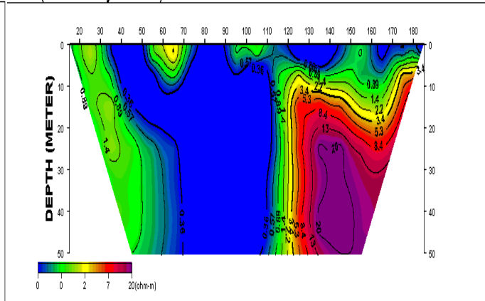
Profile (2-D Resistivity Structure)
