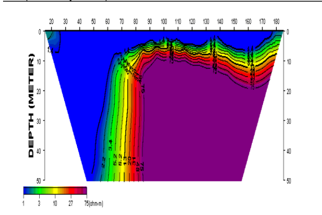
Profile (2-D Resistivity Structure)
