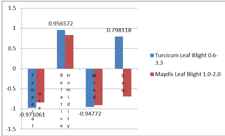
Fig 1. graphical presentation of weather parameters with disease severity
