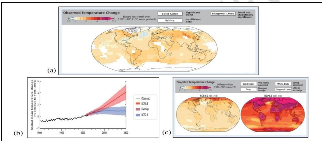
Figure2. Observed and projected changes in annual average surface temperature
