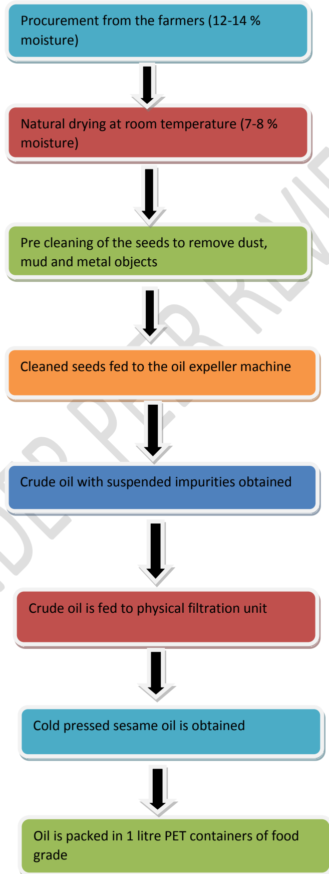
Figure 1 Process of cold pressed sesame oil extraction
