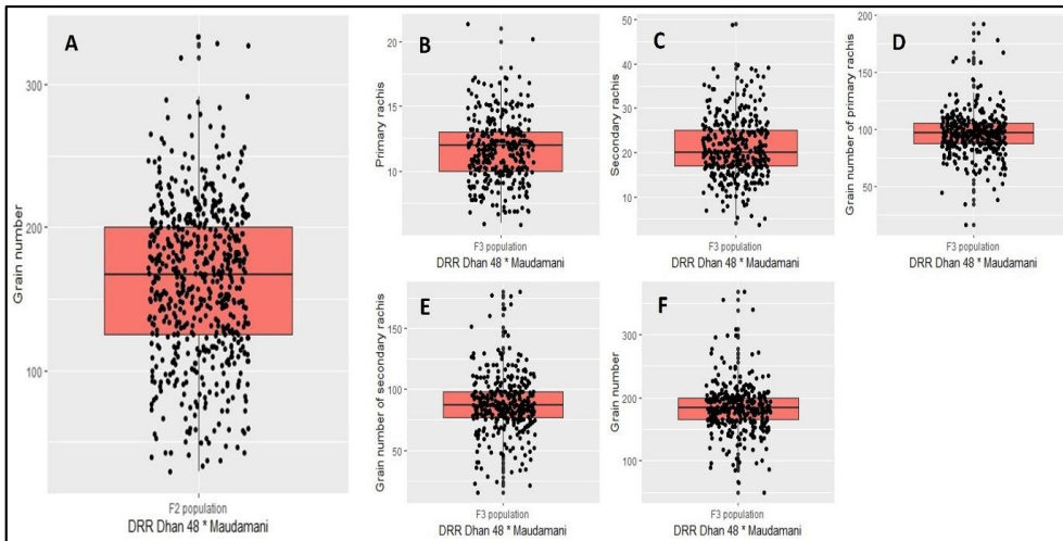
Figure 2. Box plots showing variation for panicle architecture traits in segregating populations from the cross of DRR Dhan 48/Maudamani. Box plot showing graphical representation of frequency distribution for each trait. The box indicating the existence of the 50% of the data within the box, the lower end of the box is 1 st quartile (Q1), the upper end of the box is 3 rd quartile (Q3) which shows the existence of the 25% of data above the Q3 and below the Q1, remaining 25% of the data is distributed, with solid line indicating the median value of the data distribution, the points above the outlier are the maximum value for the traits. The upper, median and lower quartiles represent the 75 th , 50 th and 25 th percentiles of the genotypes, respectively. The vertical lines represent the variation in the population. Dots represent the outliers.
