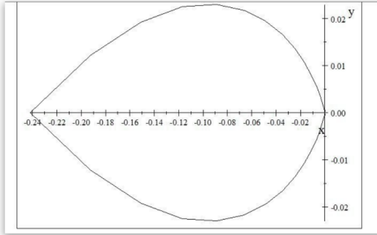
Figure 1: Region of Absolute Stability of the proposed method
