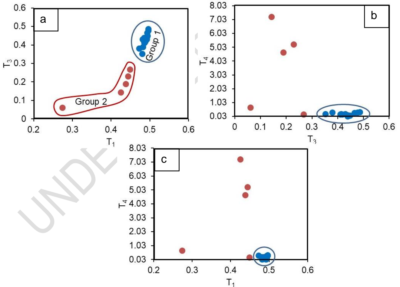
Fig. 7. Scatter plot of the size of T_3-T_1 , T_4-T_3 , T_4-T_1 tetrad effect for the stream sediment samples of Betare Oya
