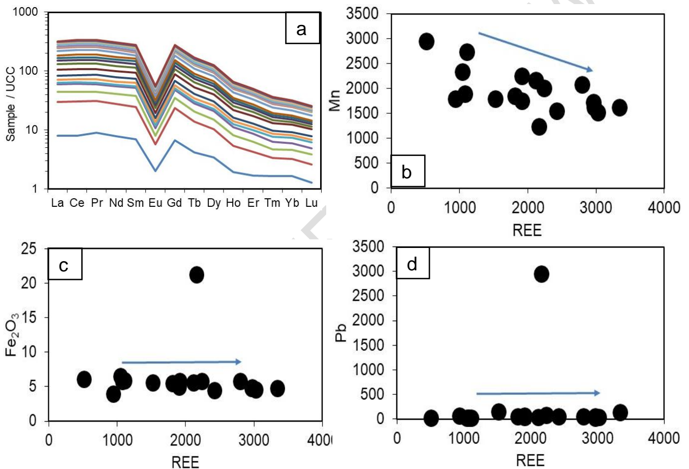
Fig. 4. REE element variation in stream sediment of Betare oya area. (a) UCC- normalized REE patterns of stream sediment samples from Betare Oya, normalization standards from [10]; (b-d) bivariate plots of \text{Fe}_2\text{O}_3 , Mn and Pb relative to REE
