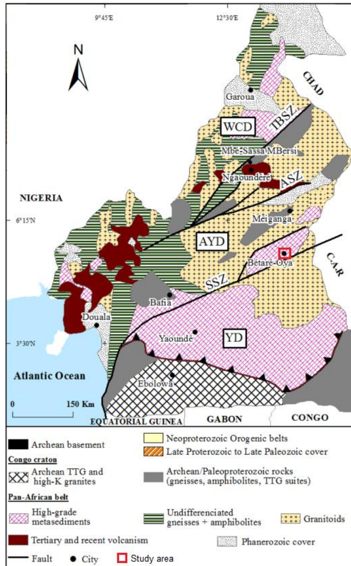
Fig. 1. Geological map of Cameroon showing the study area. ASZ Adamawa Shear Zone, YD: Yaoundé Domain, AYD: Adamawa-Yadé Domain, WCD: Western Cameroon Domain, SSZ: Sanaga Shear Zone, TBSZ: Tchollire-Banyo Shear Zone [14]
