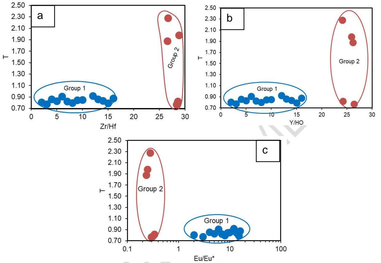
Fig. 10. Plots of \text{Eu}/\text{Eu}^* , \text{Zr}/\text{Hf} and \text{Y}/\text{Ho} against the degree of the tetrad effect (T)
