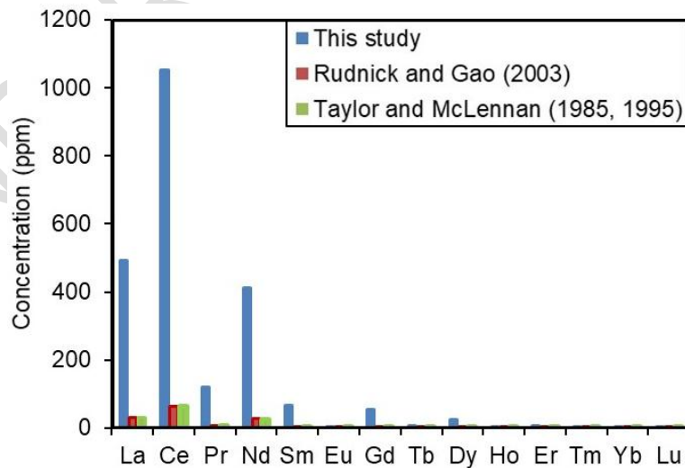
Fig. 11. Graphical representation of the mean concentration of REE in stream sediment of Betare Oya in comparison to the values of the UCC by [21, 34]
