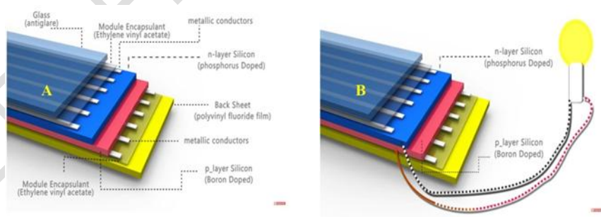
Figure 3: Configuration and working of solar photovoltaic (PV) cell
