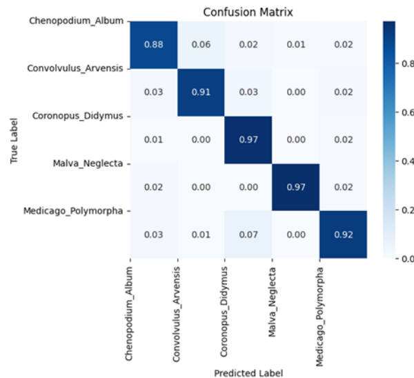
Fig 2. Confusion matrix of weed identification model
