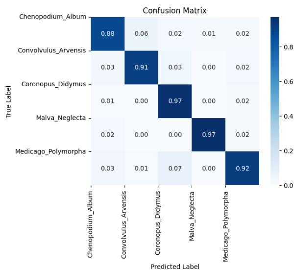
Fig 1. Confusion matrix of weed identification model
