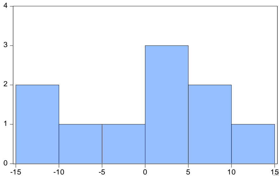
Figure 2: Normality Test
