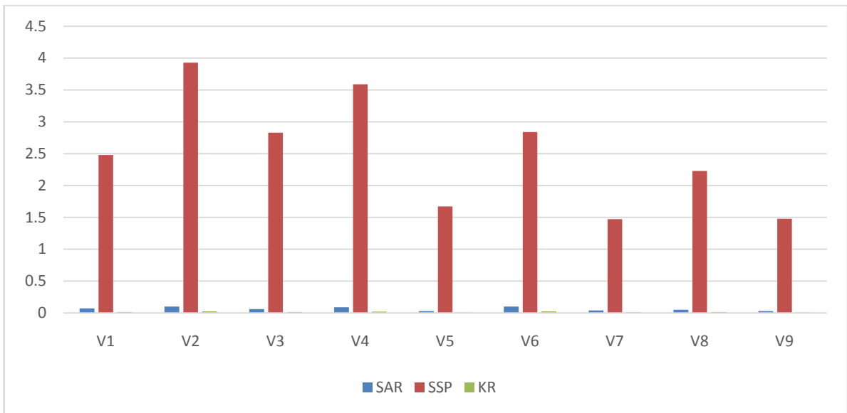
Fig 8: SAR, SSP and KR of Irrigation Water Quality Parameters of Phulpur block in Prayagraj district
