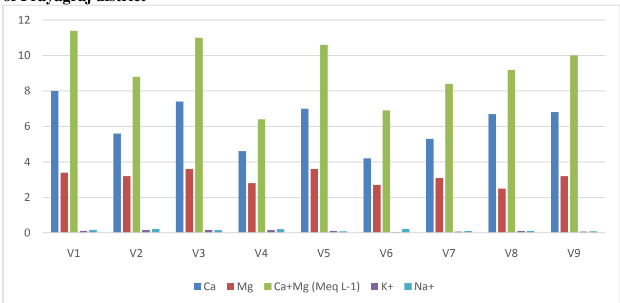
Fig.7: Ca, Mg, Ca+Mg, K + and Na + of water sample different villages of Phulpur block of Prayagraj district
