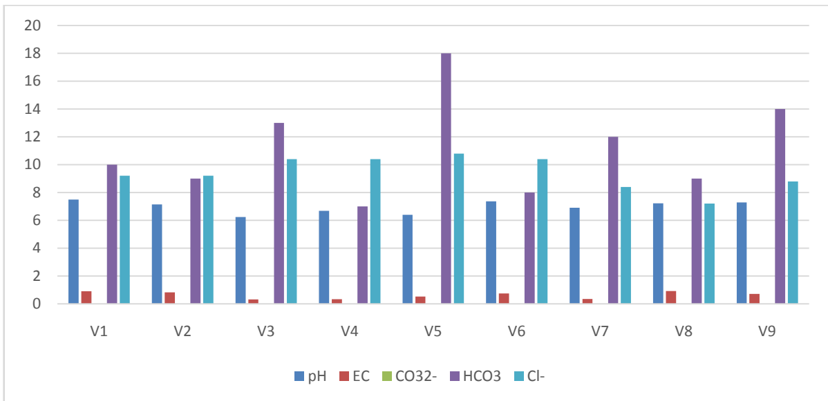
Fig.6: pH, EC, CO 3 2- , HCO 3 and Cl - of water sample different villages of Phulpur block of Prayagraj district
