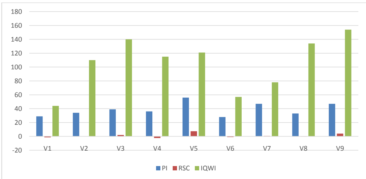
Fig 9: PI, RSC and IQWI of Irrigation Water Quality Parameters of Phulpur block in Prayagraj district
