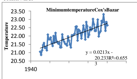
(d) Time Series plot with trend of minimum temperature of Cox's Bazar
