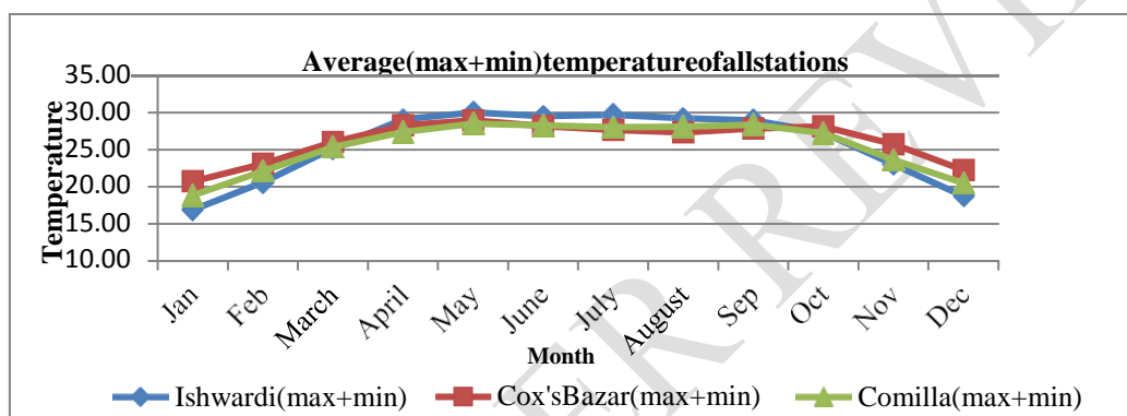
Fig.7Frequencycurve foraverage(max + min)temperatureofallthreestations
