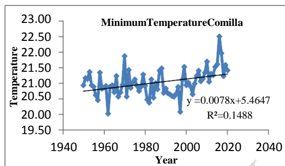
(f) Time Series plot with trend of minimum temperature of Comilla
