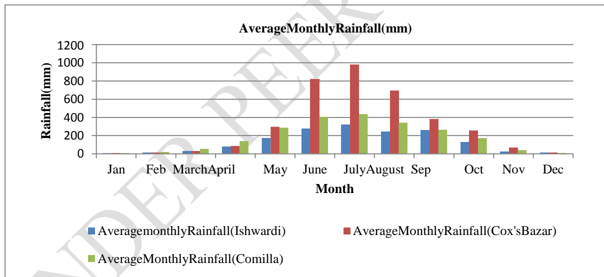
Fig.8 Multiple bar diagram for average monthly rainfall (mm)
