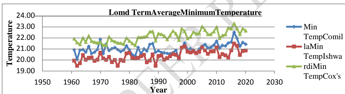
Fig.6 Long term average Minimum temperature
