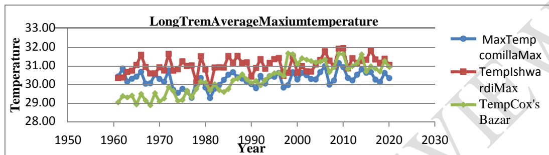
Fig.5 Long term average Maximum temperature
