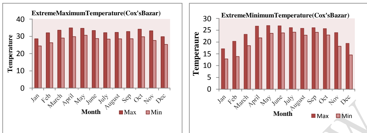
Fig.3 Bar diagram showing extreme maximum and minimum temperature of Cox's Bazar
