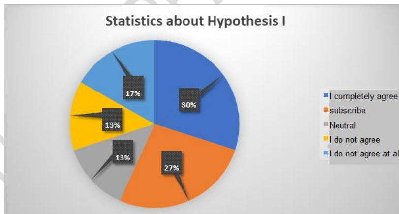
Figure 1549. Graph for Hypothesis statistics
