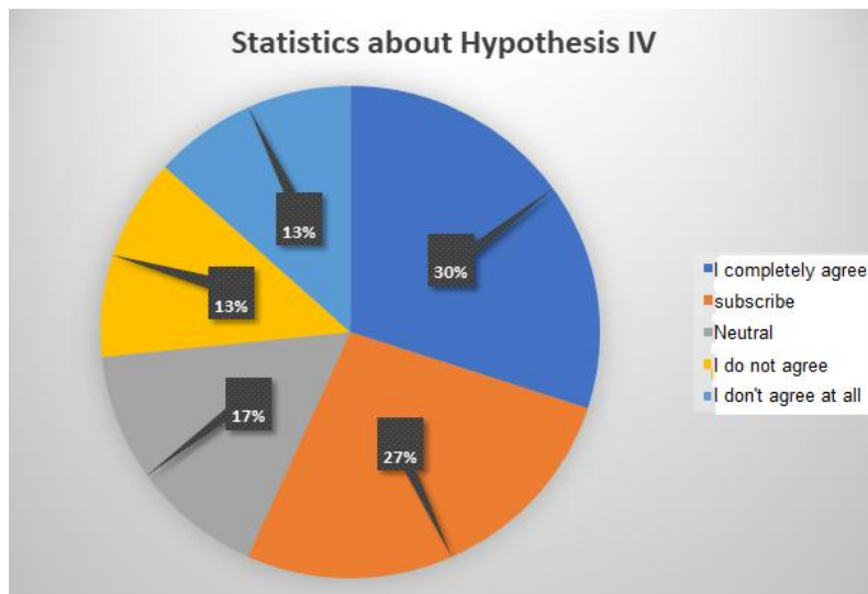
Figure 1822. Graph for Hypothesis IV statistics
