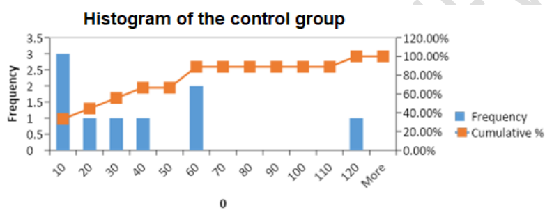
Figure 13+7. Histogram of the control group
