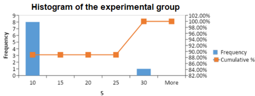
Figure 12+6. Histogram of the experimental group
