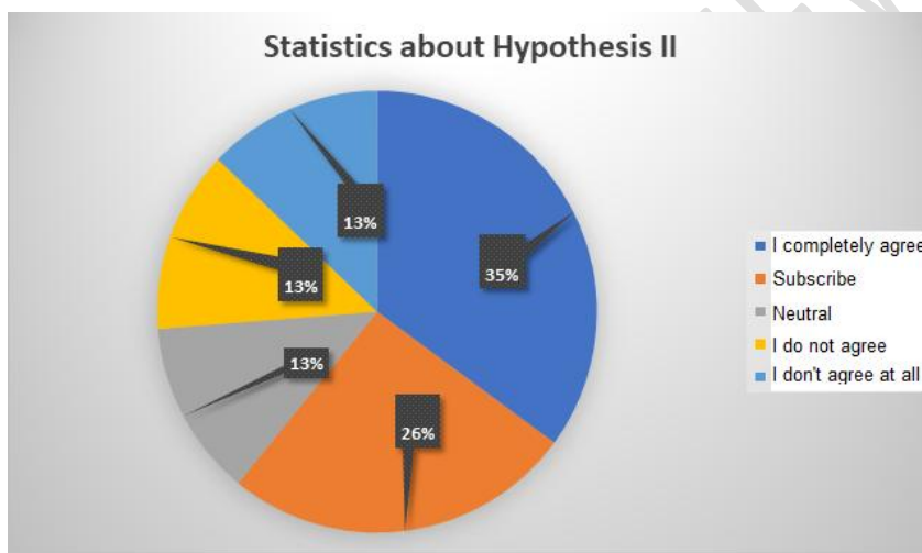
Figure 1620. Graph for Hypothesis II statistics
