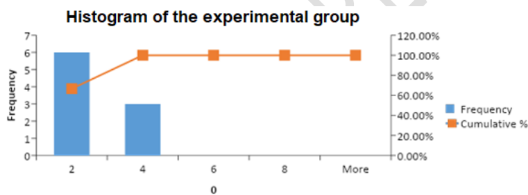
Figure 1418. Histogram of experimental set- Error measurement variable
