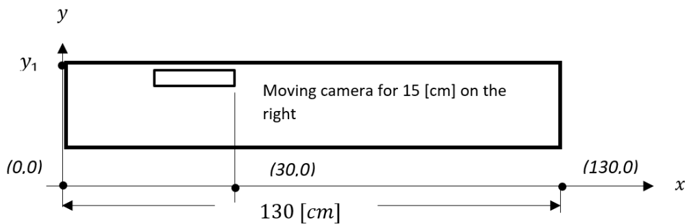
Figure 4. Moving the camera for 15 [cm] on the right
