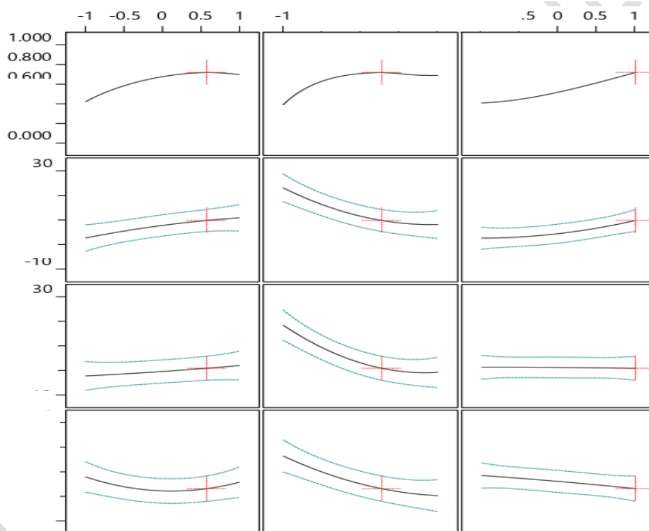
Fig. 2. Factors plot of optimum conditions of the extraction yield (%), acid value (mg of KOH/g) and peroxide value (meq of O 2 //kg).
