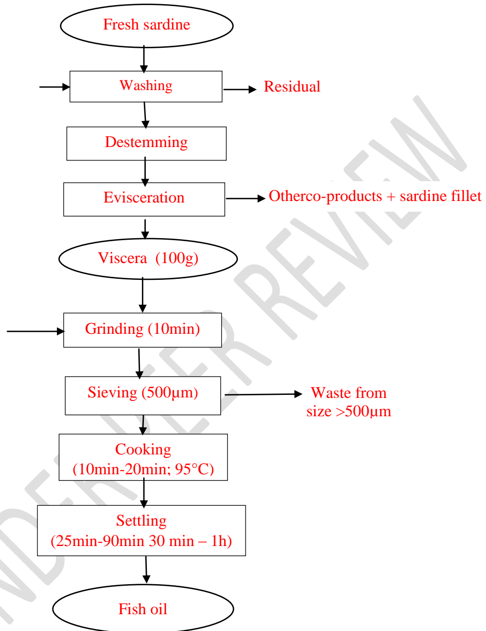
Fig. 1. Flow diagram of sardine viscera oil's extraction
