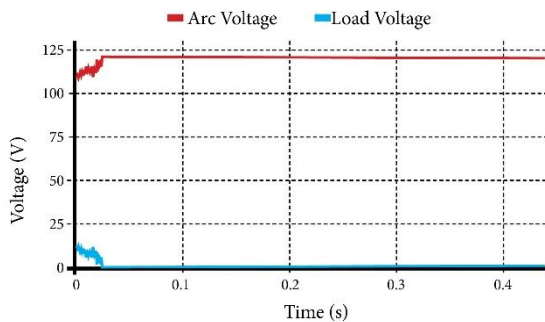
Fig. 2. Time vs Arc voltage and Load voltage (During the contact open to close switch action).
