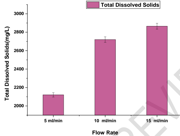
Fig.4. Influence of different hydraulic loading rate of TDS of the effluent
