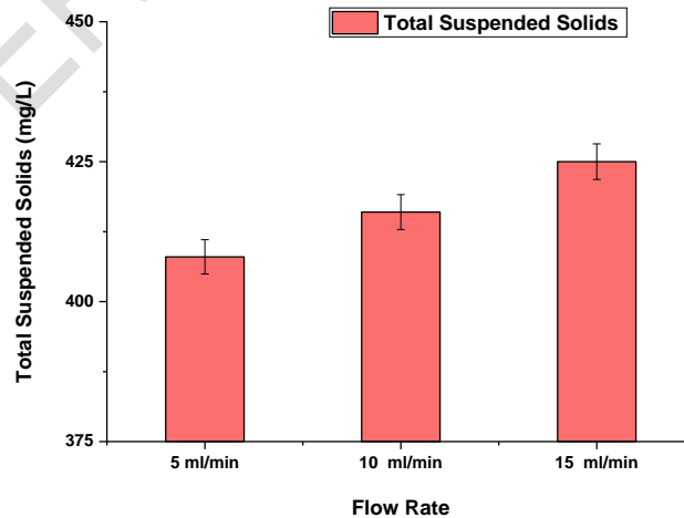
Fig.3. Influence of different hydraulic loading rate of TSS of the effluent
